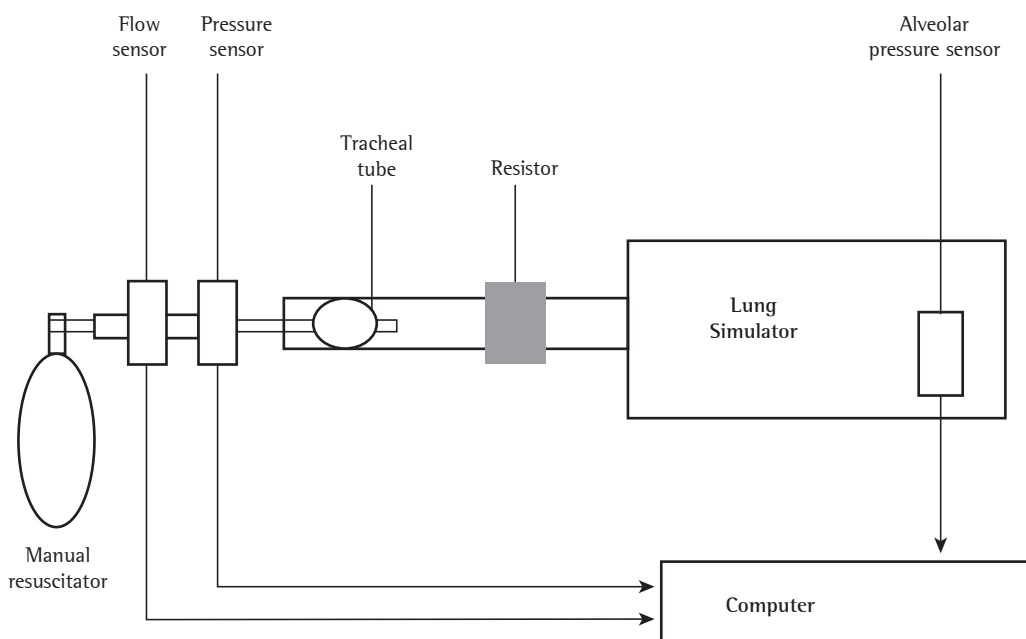
Figure 1 - Experimental setup.
